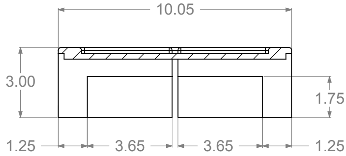
SECTION E-E
